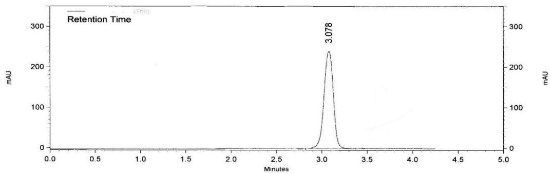
Figure 34: Chromatogram of Standard at normal condition esomeprazole
